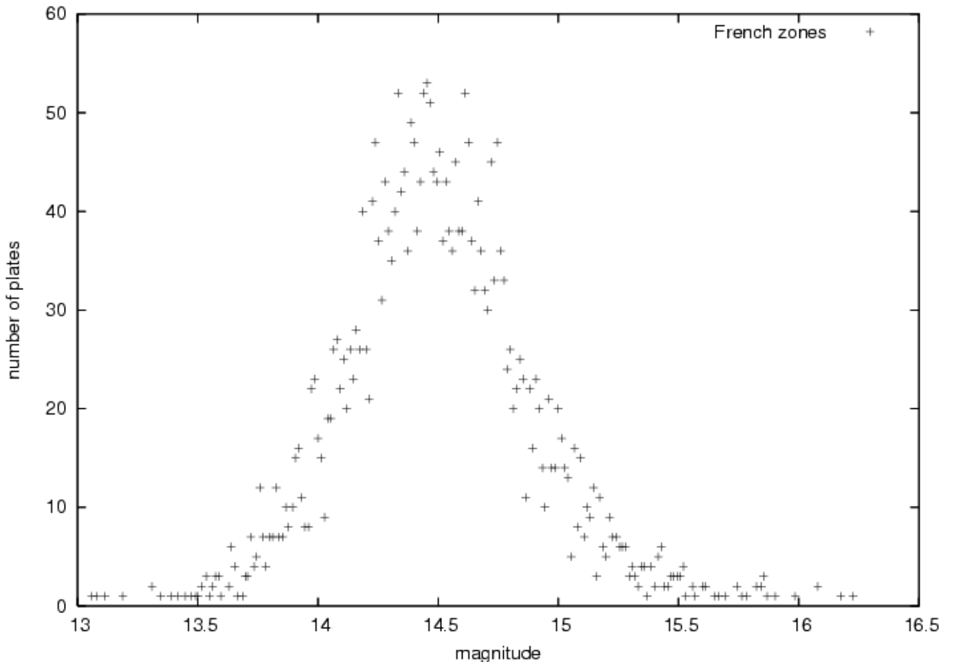
Fig. 1. Histogram of the limiting magnitude for the set of 3000 deep plates of the french zones. This magnitude is derived from the numbers of stars recorded on the skycharts and the Bahcall and Soneira's Galaxy model for stellar counts
